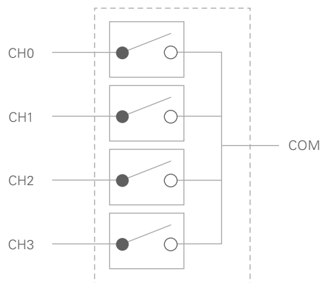
FIG 11 4 x 1 multiplexer built from multiple Form A SPST relays tied together
