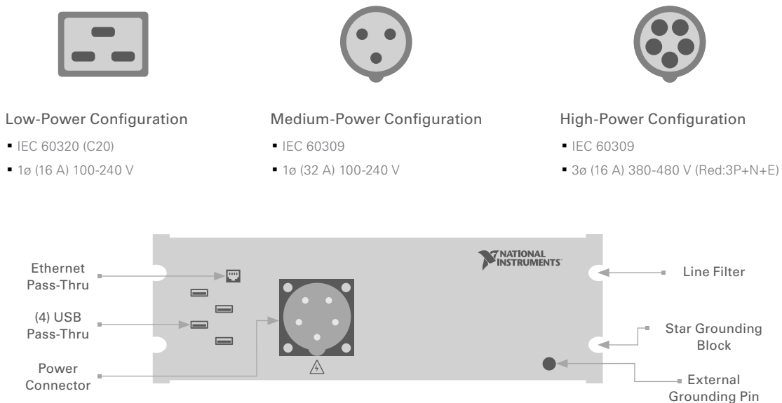
FIG 2 | A power entry panel provides connectivity for incoming power to the system. Power entry panels can have one of a number of standard power connector types and good power panels have additional features like filtering or kill-switch relays.
