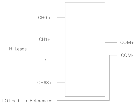
FIG 27 | Single-ended multiplexers are great for measurements that reference a shared signal or ground.
