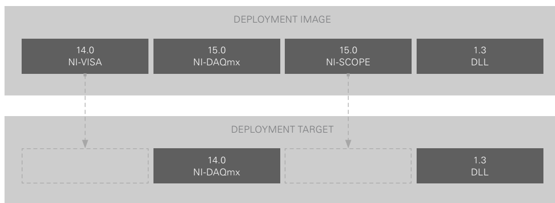
FIG 5 | Dependency assertion
